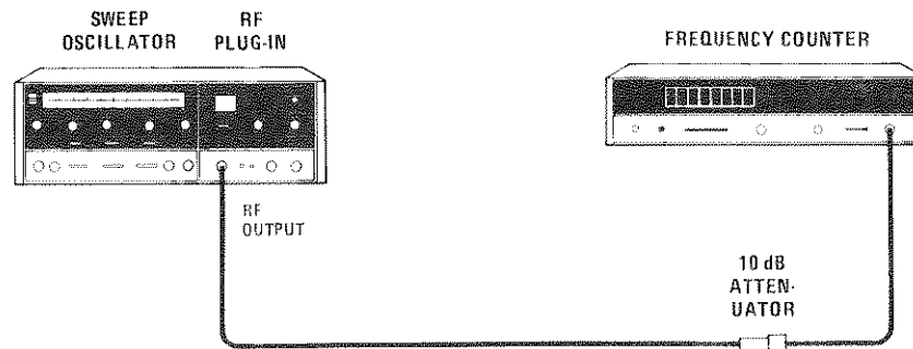
Figure 4-1. CW Vernier Test Setup
