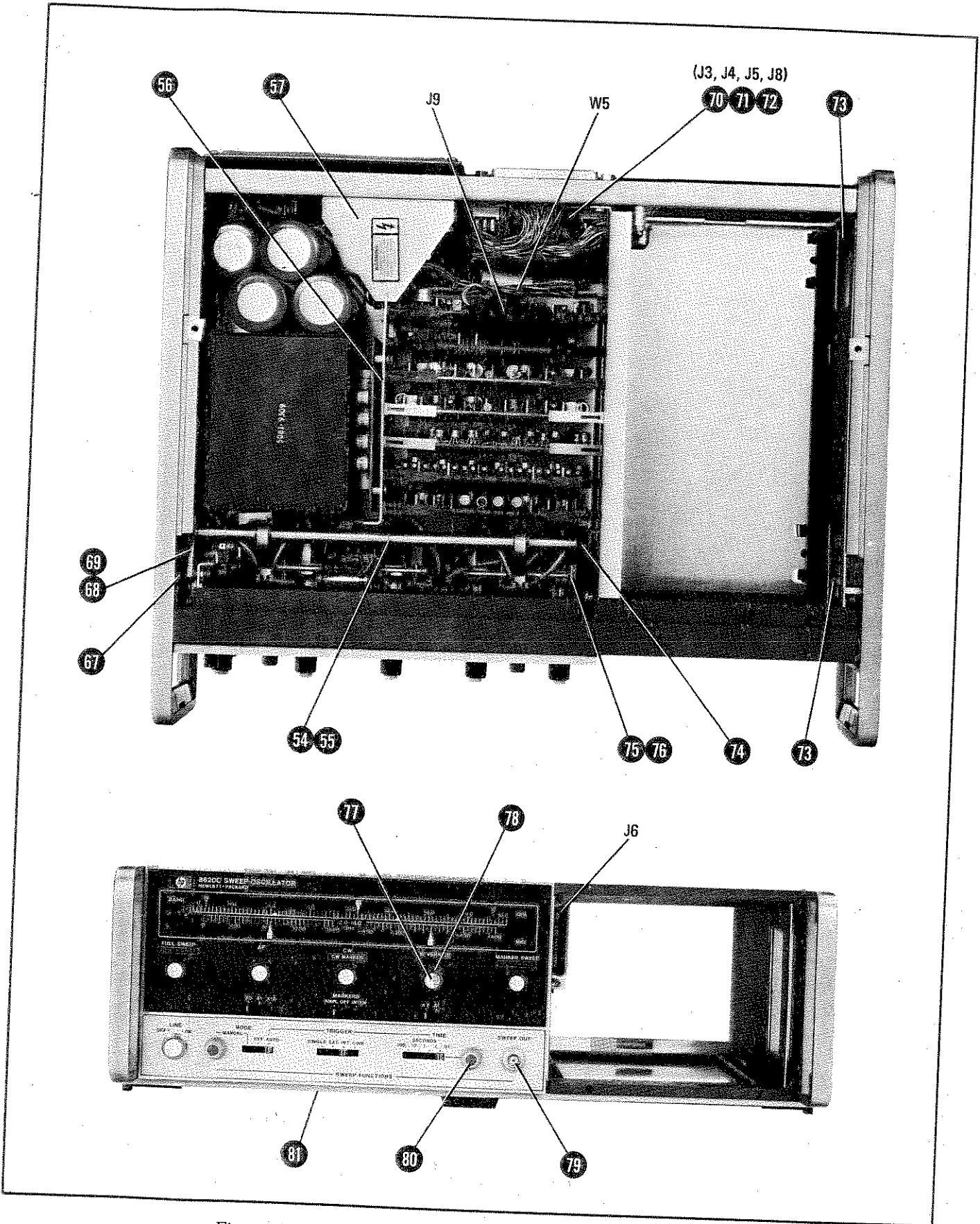
Figure 6-1. Front Panel Assembly, Parts Locations (4 of 4)
