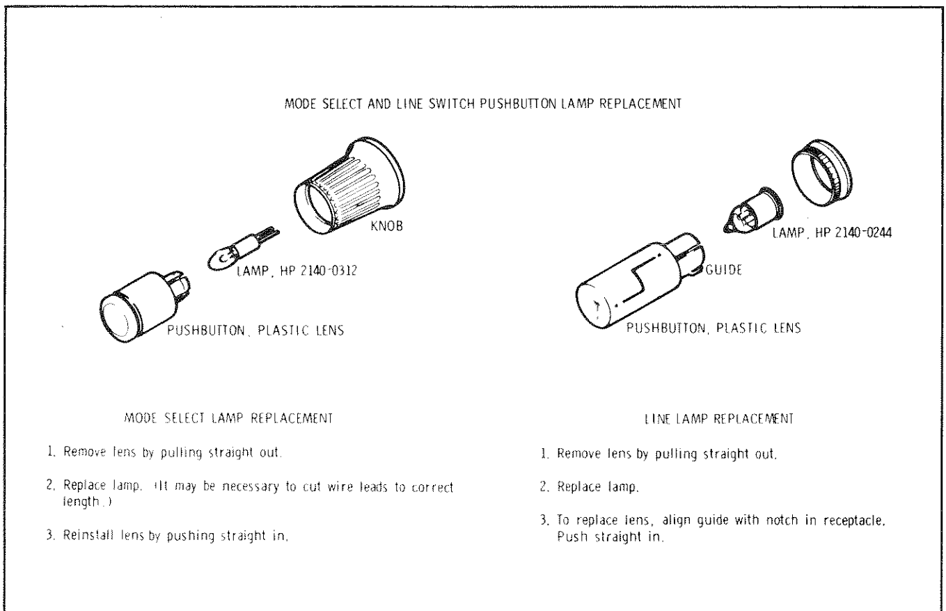
Figure 3-3. Lamp Replacement
