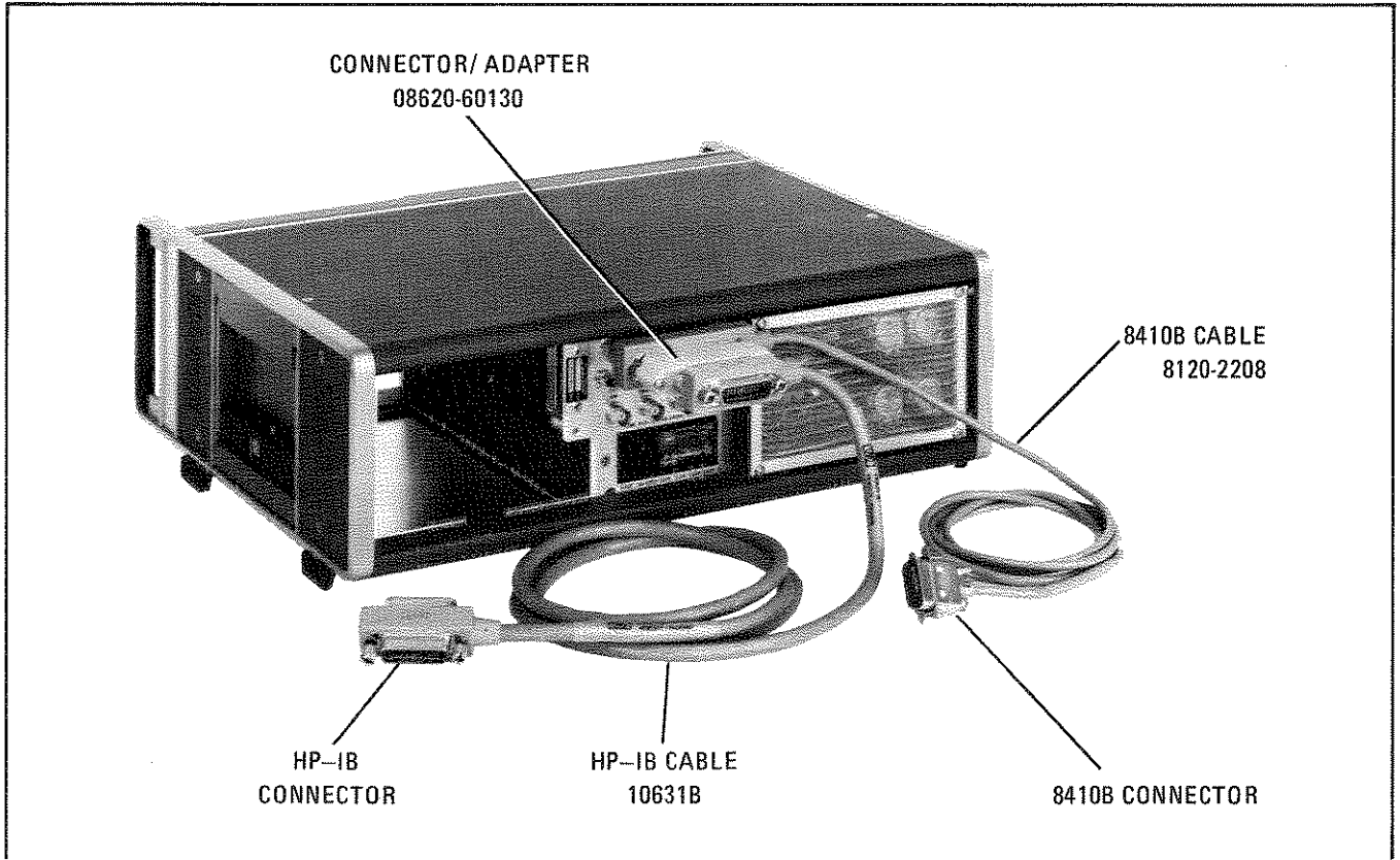
Figure 2-9. HP-IB/8410B Installation
